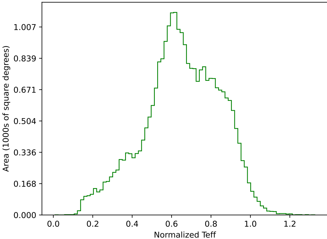
baseline_v3.0_10yrs All sky g band: Normalized Teff
