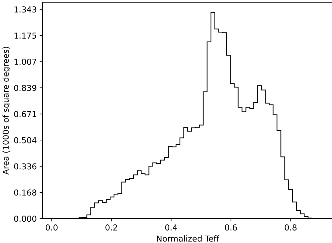
baseline_v3.0_10yrs All sky all bands: Normalized Teff
