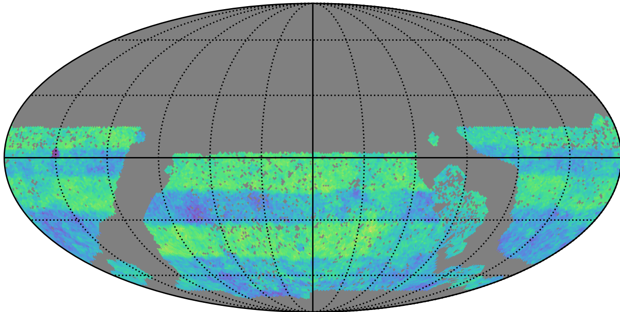
baseline_v3.0_10yrs WFD: Normalized Proper Motion Uncert @ 24.0
