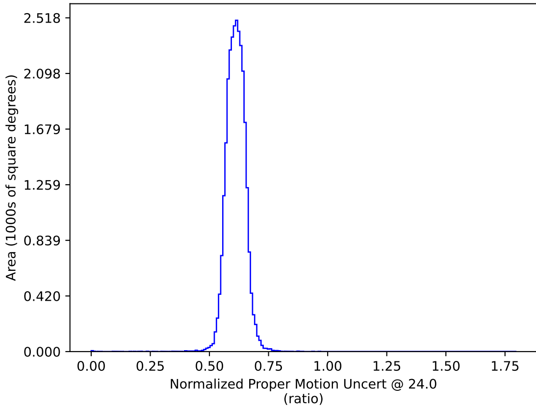
baseline_v3.0_10yrs All sky: Normalized Proper Motion Uncert @ 24.0
