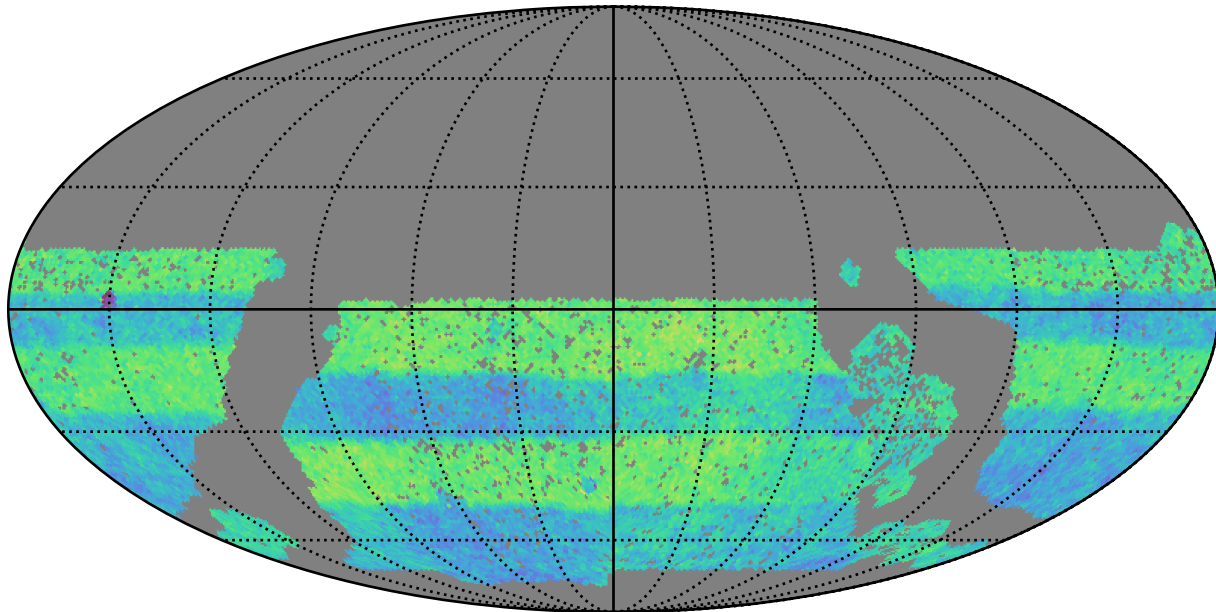
baseline_v3.0_10yrs WFD: Normalized Proper Motion Uncert @ 20.5
