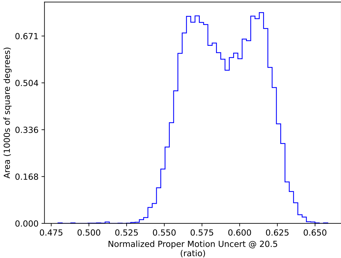
baseline_v3.0_10yrs WFD: Normalized Proper Motion Uncert @ 20.5
