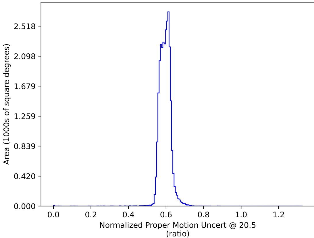
baseline_v3.0_10yrs All sky: Normalized Proper Motion Uncert @ 20.5
