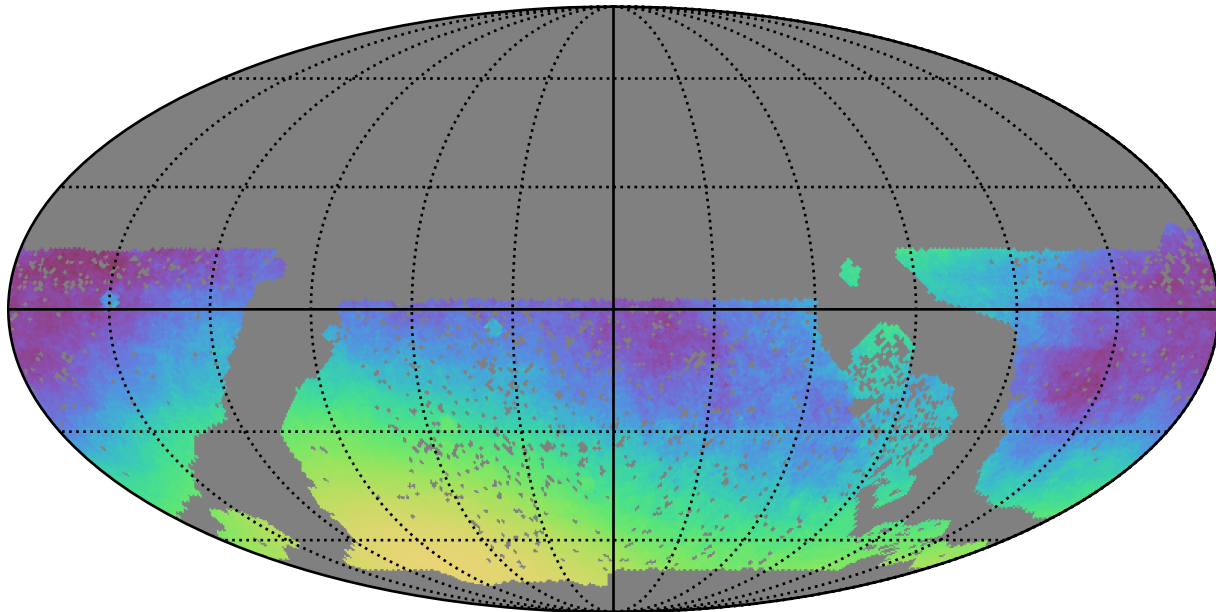
baseline_v3.0_10yrs WFD: Normalized Parallax Uncert @ 24.0
