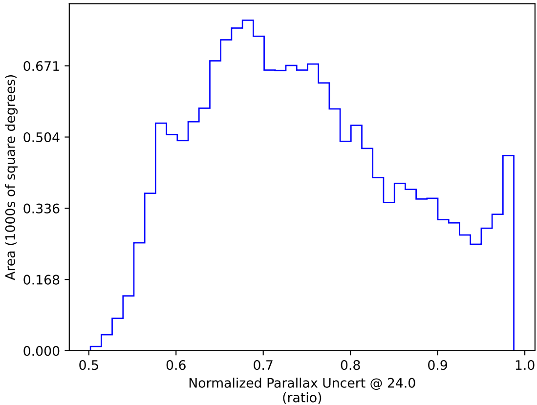
baseline_v3.0_10yrs WFD: Normalized Parallax Uncert @ 24.0
