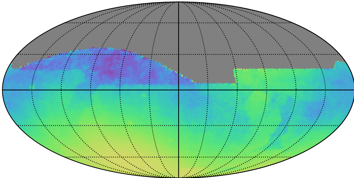
baseline_v3.0_10yrs All sky: Normalized Parallax Uncert @ 24.0
