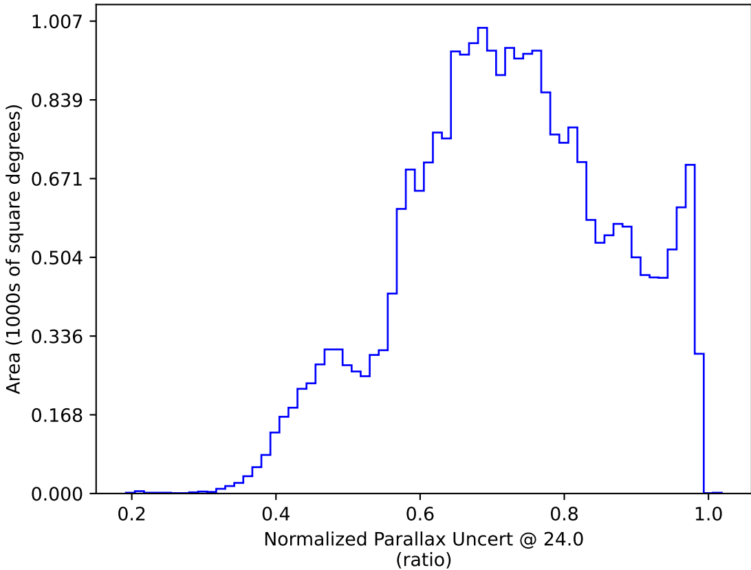
baseline_v3.0_10yrs All sky: Normalized Parallax Uncert @ 24.0
