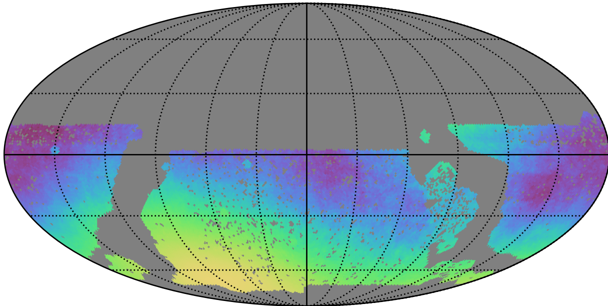
baseline_v3.0_10yrs WFD: Normalized Parallax Uncert @ 22.4
