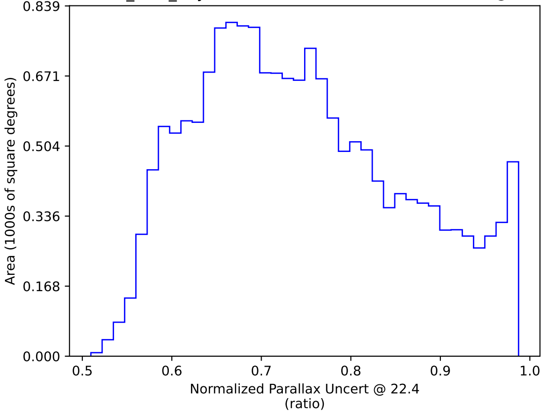
baseline_v3.0_10yrs WFD: Normalized Parallax Uncert @ 22.4
