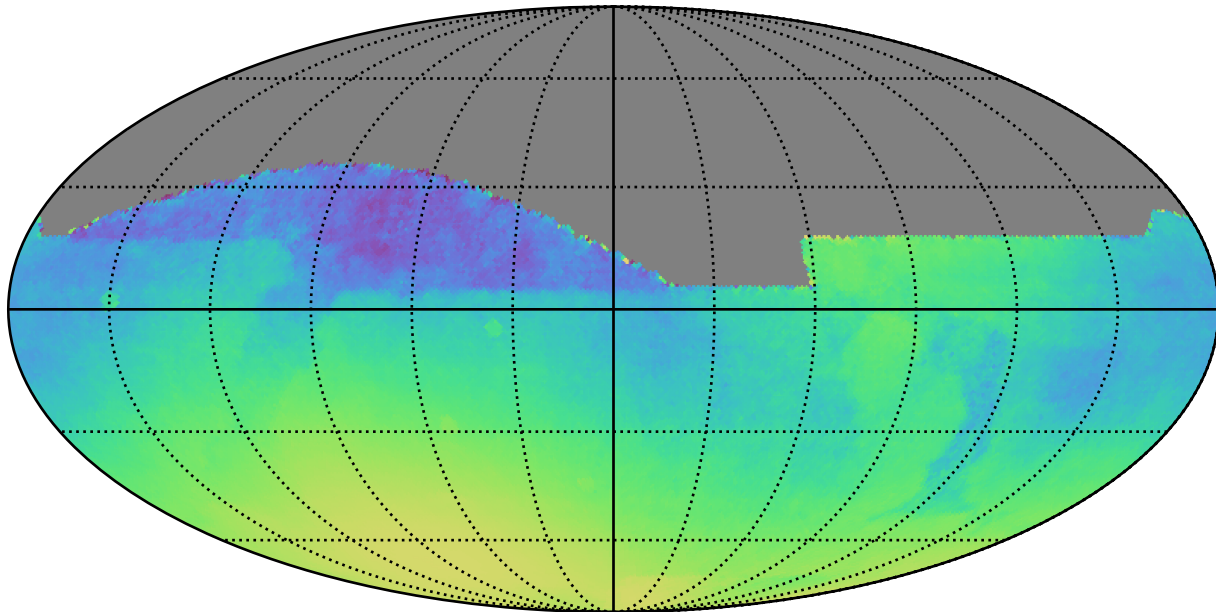
baseline_v3.0_10yrs All sky: Normalized Parallax Uncert @ 22.4
