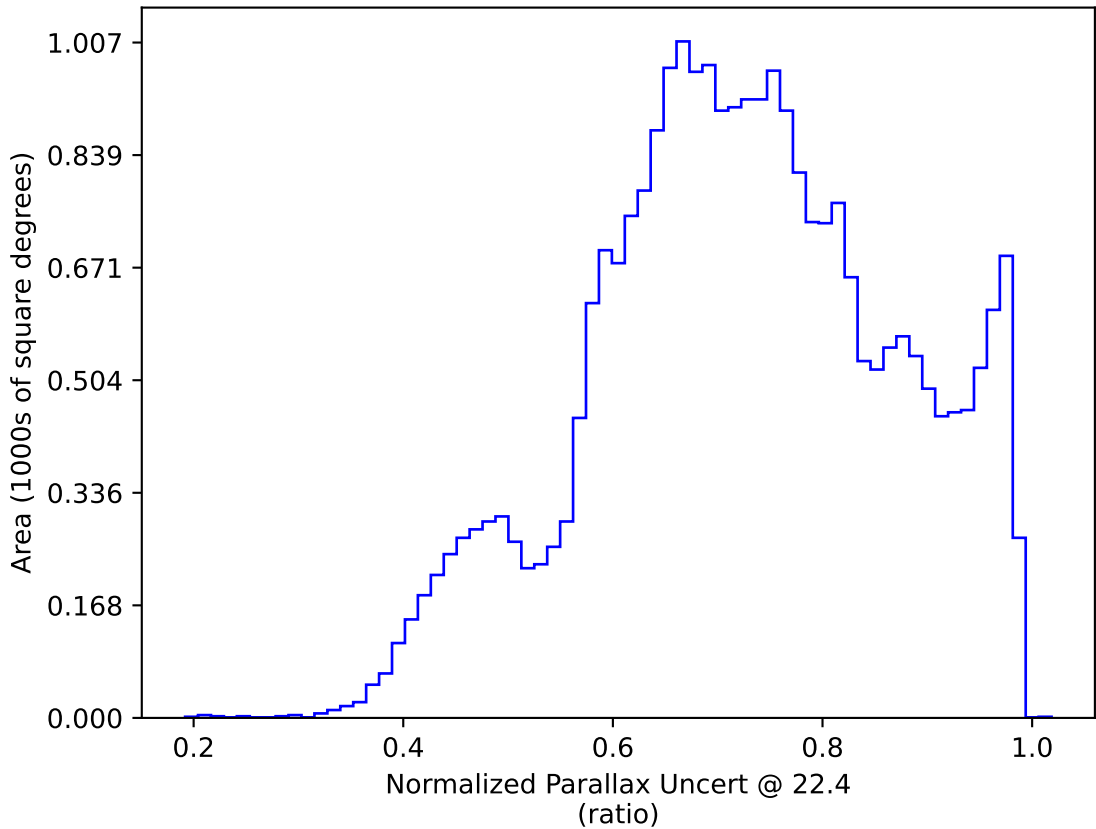
baseline_v3.0_10yrs All sky: Normalized Parallax Uncert @ 22.4
