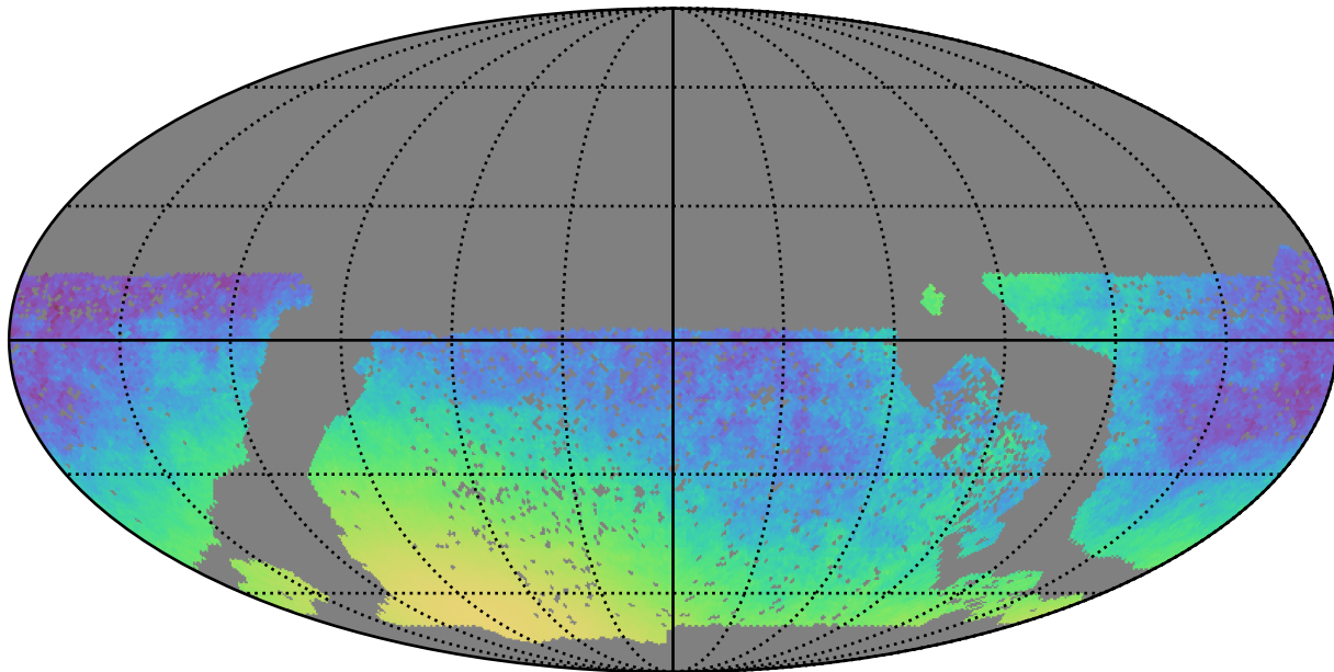
baseline_v3.0_10yrs WFD y band only: Normalized Parallax Uncert @ 21.3
