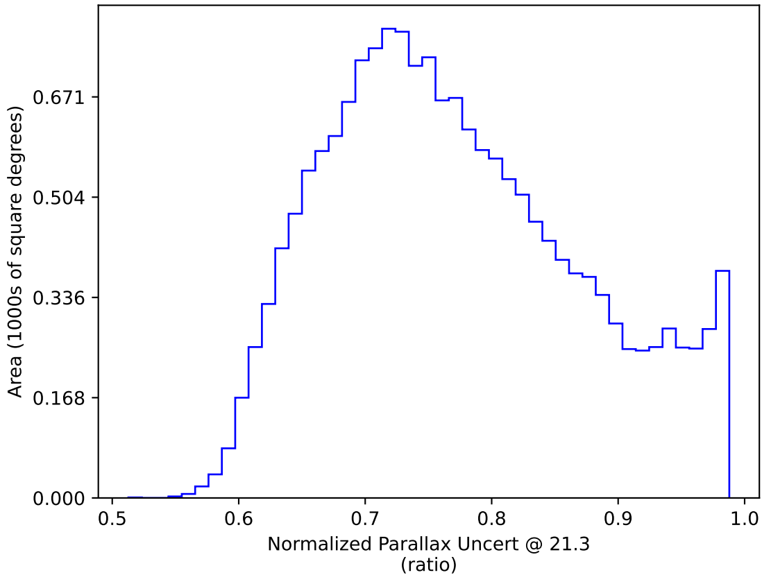
baseline_v3.0_10yrs WFD y band only: Normalized Parallax Uncert @ 21.3
