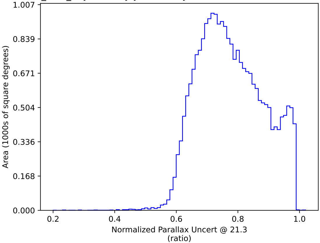
baseline_v3.0_10yrs All sky y band only: Normalized Parallax Uncert @ 21.3
