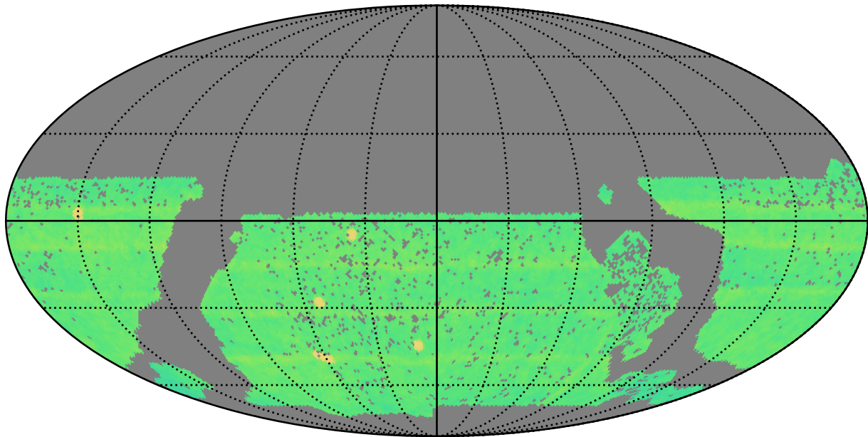
baseline_v3.0_10yrs WFD all bands: N Unique Nights
