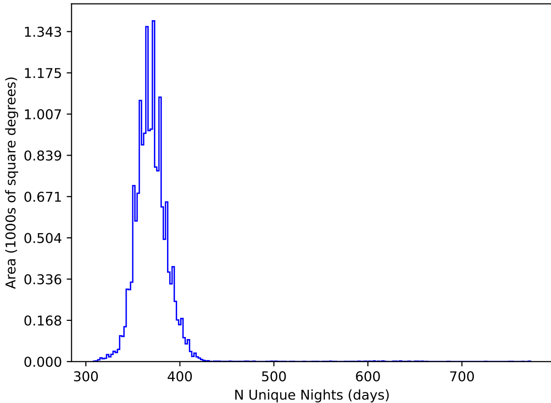
baseline_v3.0_10yrs WFD all bands: N Unique Nights
