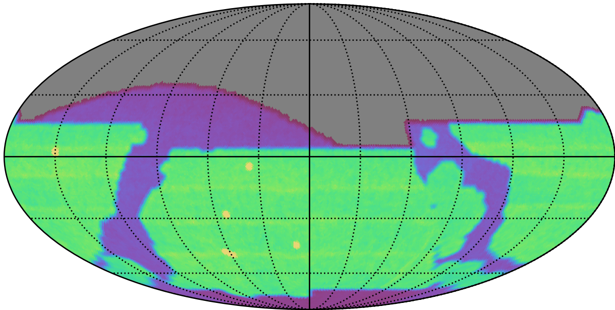
baseline_v3.0_10yrs All sky all bands: N Unique Nights
