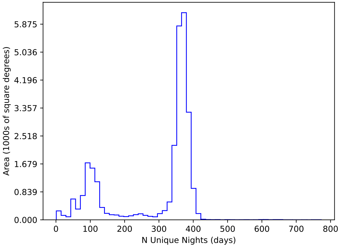
baseline_v3.0_10yrs All sky all bands: N Unique Nights
