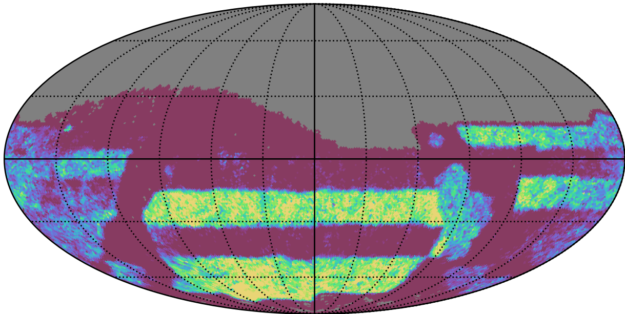
baseline_v3.0_10yrs Yr 3-4 z band: NVisits
