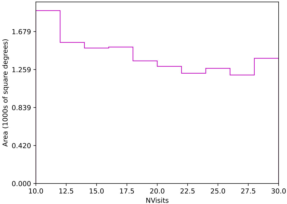
baseline_v3.0_10yrs Yr 3-4 z band: NVisits
