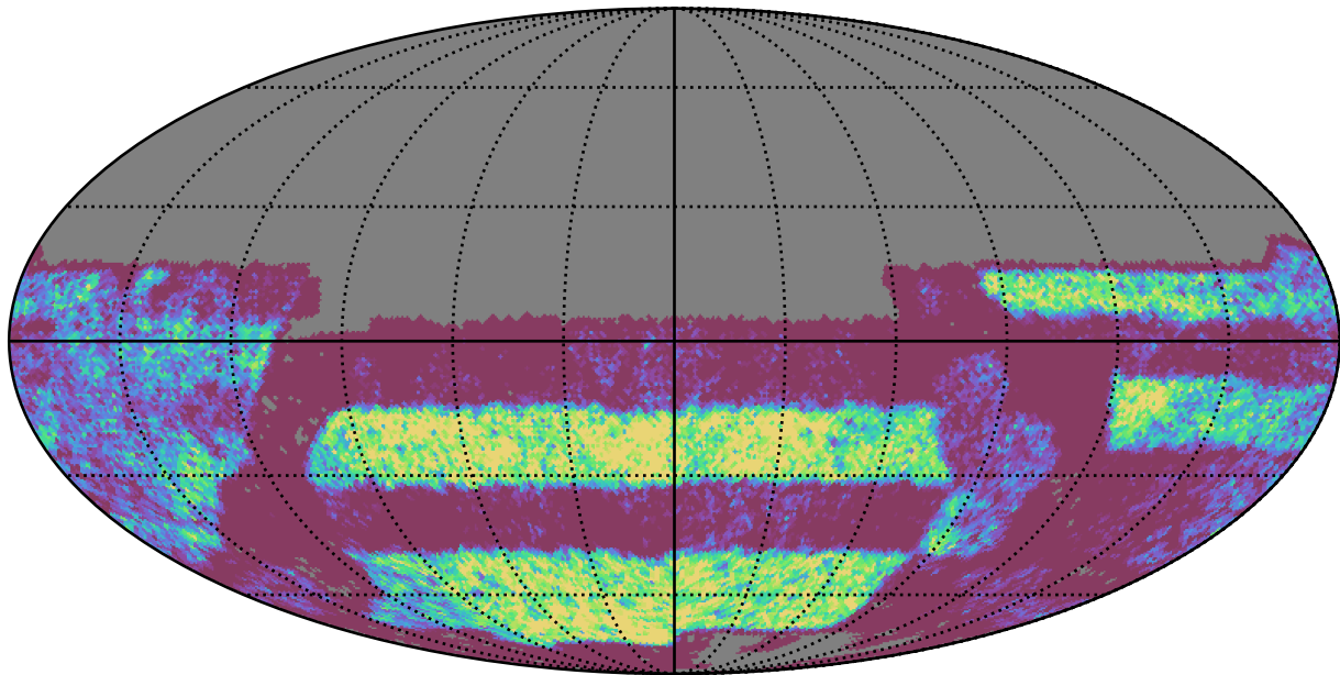
baseline_v3.0_10yrs Yr 3-4 y band: NVisits
