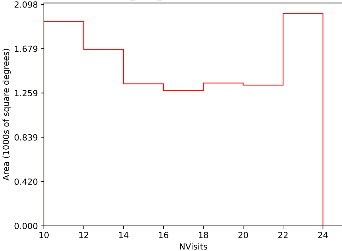
baseline_v3.0_10yrs Yr 3-4 i band: NVisits
