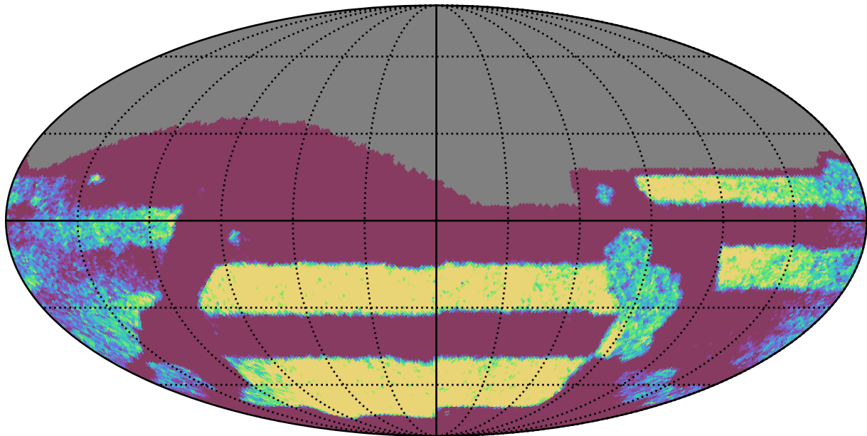
baseline_v3.0_10yrs Yr 3-4 all bands: NVisits
