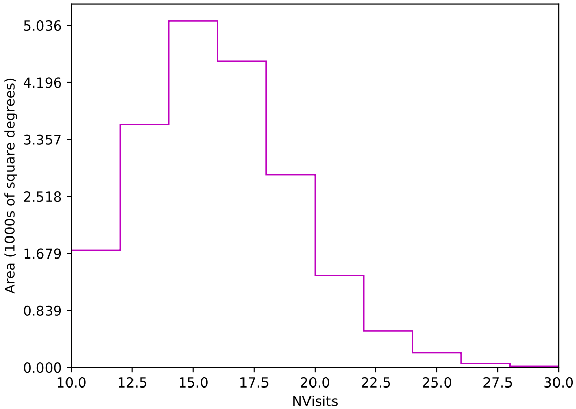
baseline_v3.0_10yrs Yr 1 z band: NVisits
