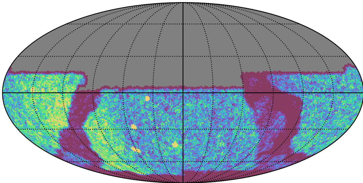
baseline_v3.0_10yrs Yr 1 y band: NVisits
