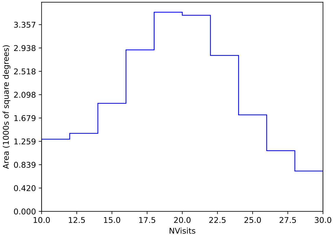
baseline_v3.0_10yrs Yr 1 y band: NVisits
