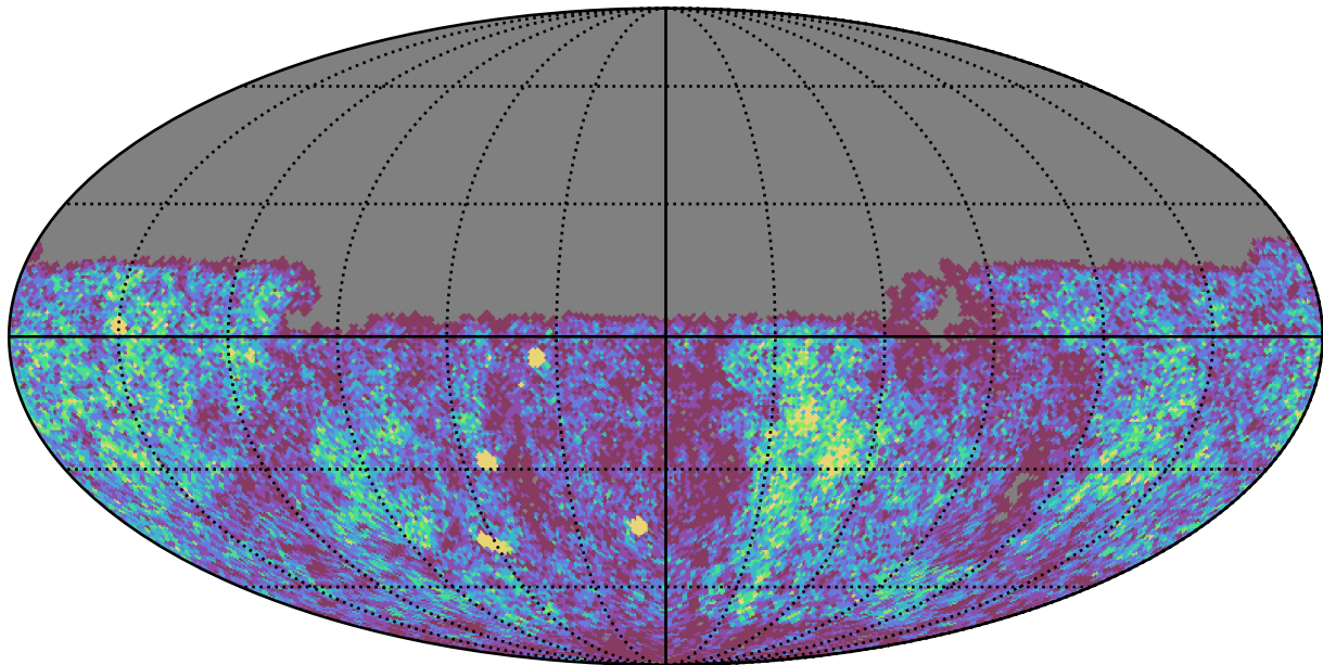
baseline_v3.0_10yrs Yr 1 u band: NVisits
