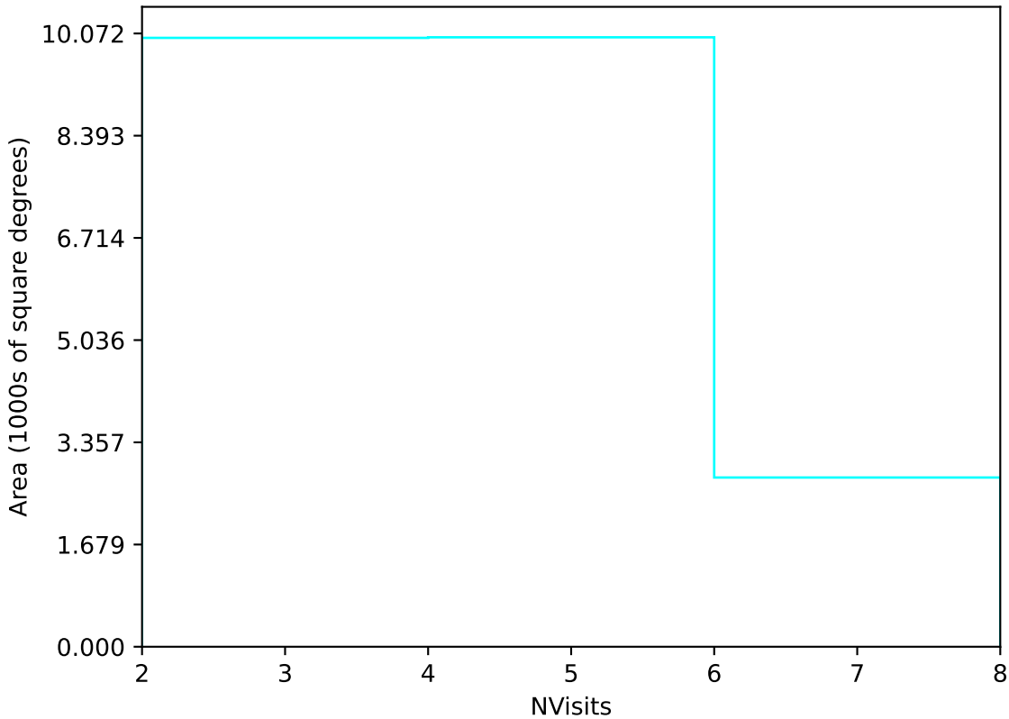
baseline_v3.0_10yrs Yr 1 u band: NVisits
