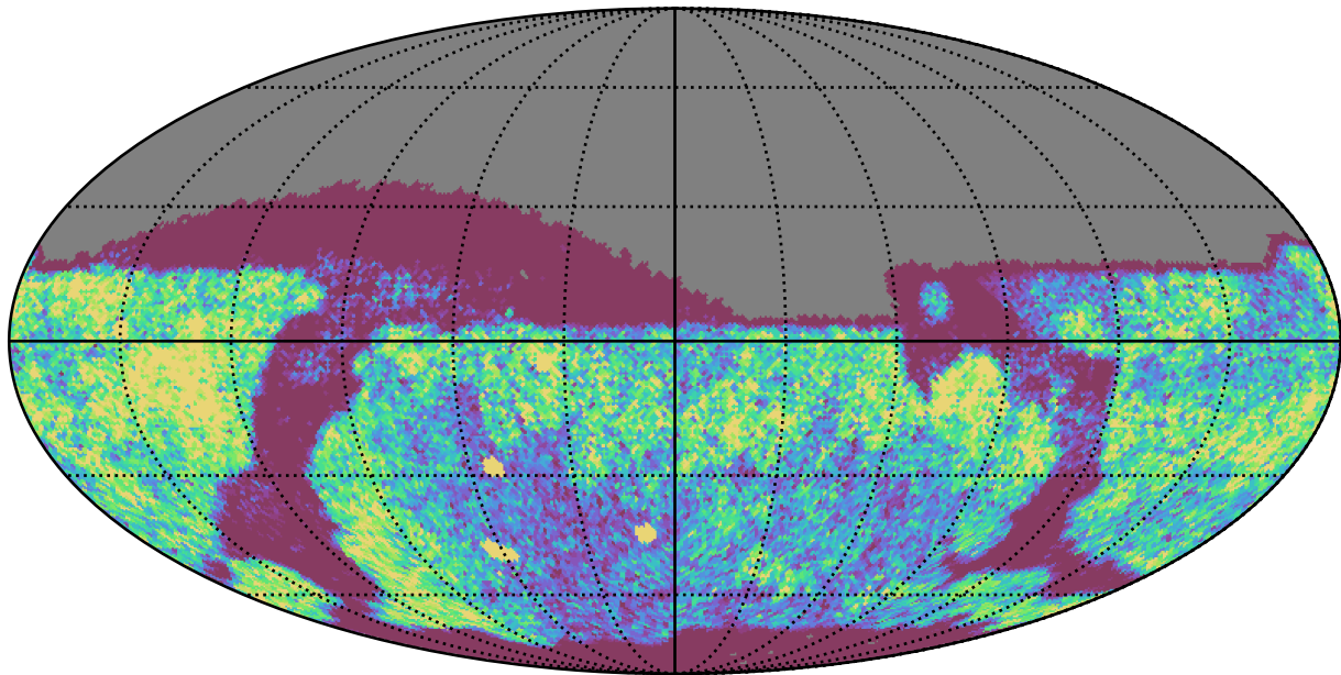
baseline_v3.0_10yrs Yr 1 r band: NVisits
