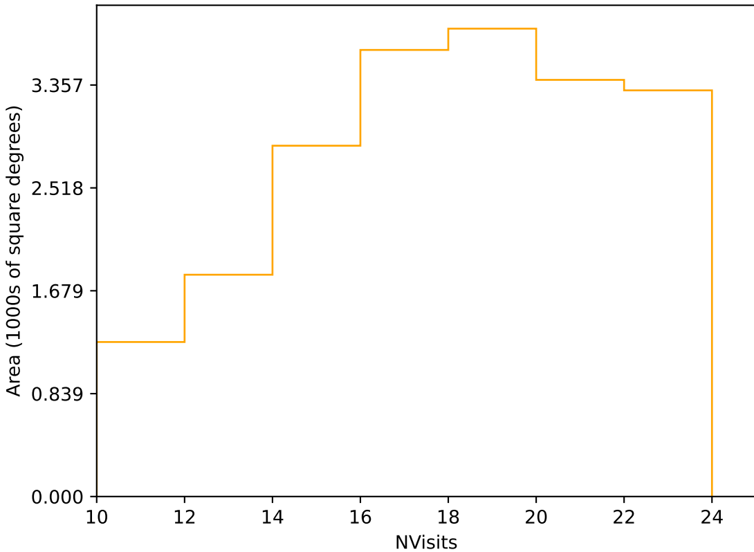
baseline_v3.0_10yrs Yr 1 r band: NVisits
