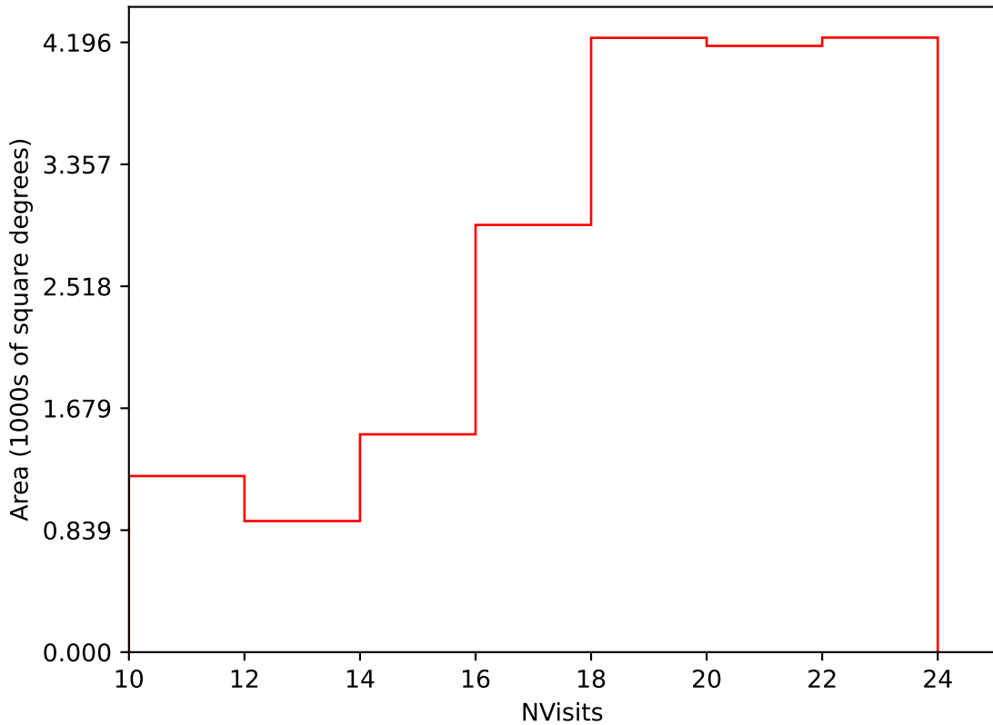
baseline_v3.0_10yrs Yr 1 i band: NVisits
