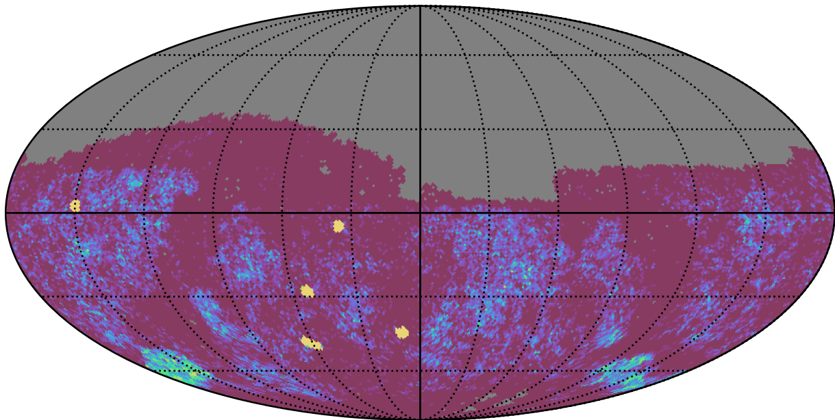
baseline_v3.0_10yrs Yr 1 g band: NVisits
