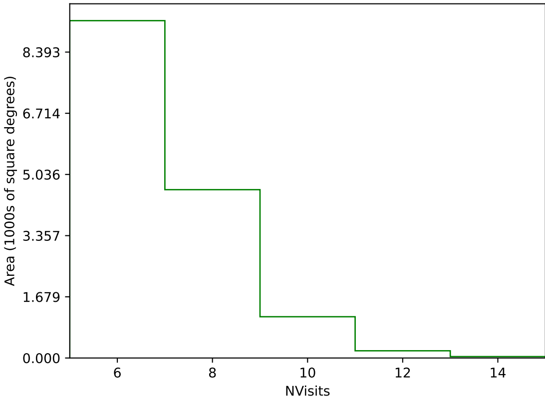
baseline_v3.0_10yrs Yr 1 g band: NVisits
