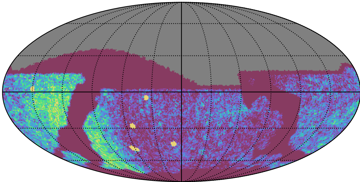
baseline_v3.0_10yrs Yr 1 all bands: NVisits
