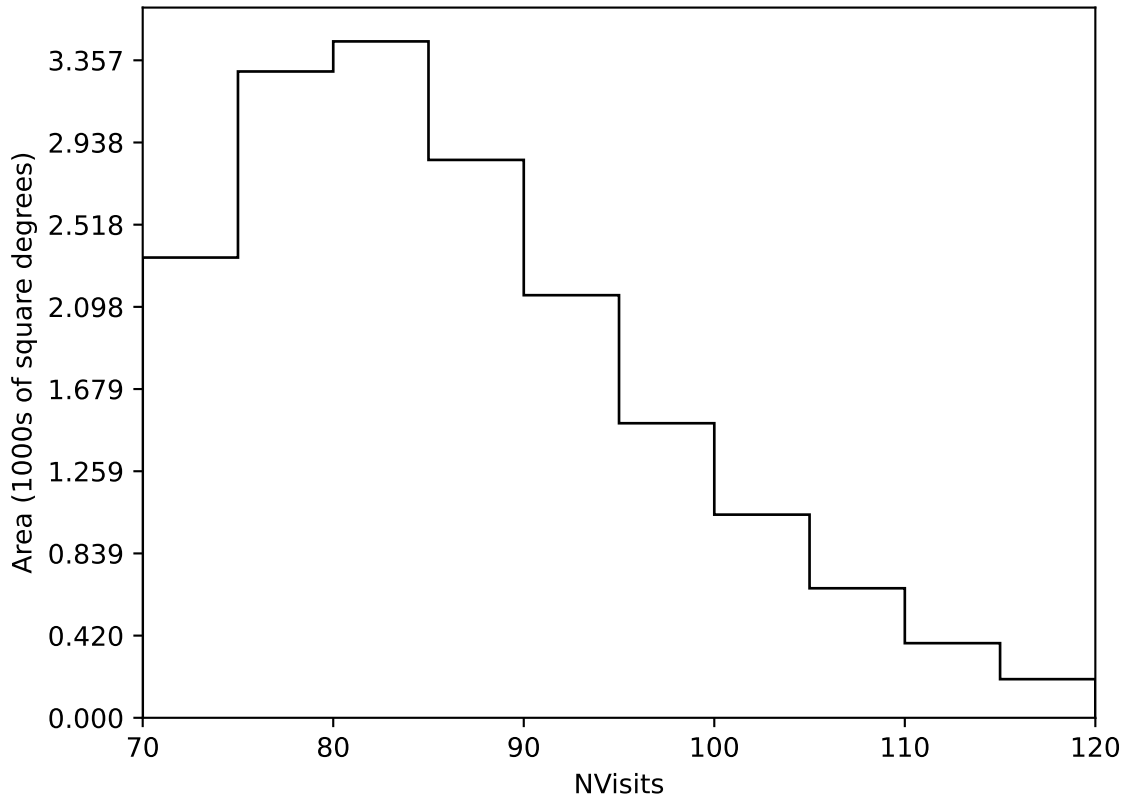
baseline_v3.0_10yrs Yr 1 all bands: NVisits
