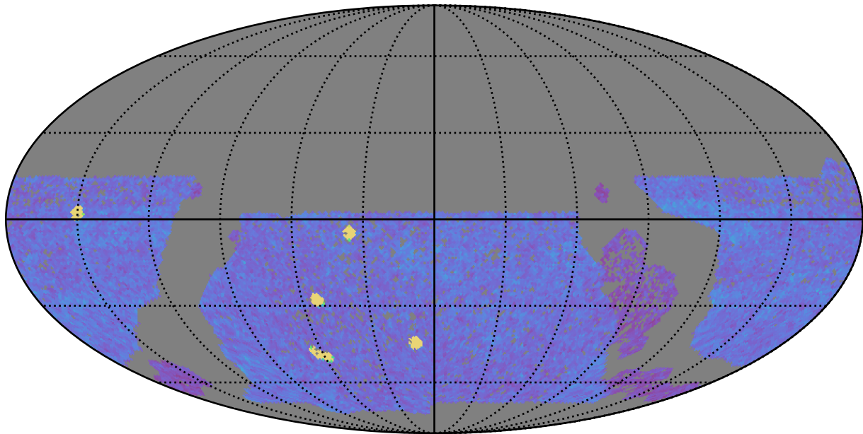
baseline_v3.0_10yrs WFD z band: NVisits
