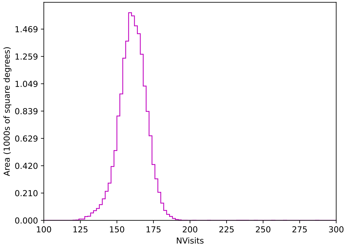
baseline_v3.0_10yrs WFD z band: NVisits
