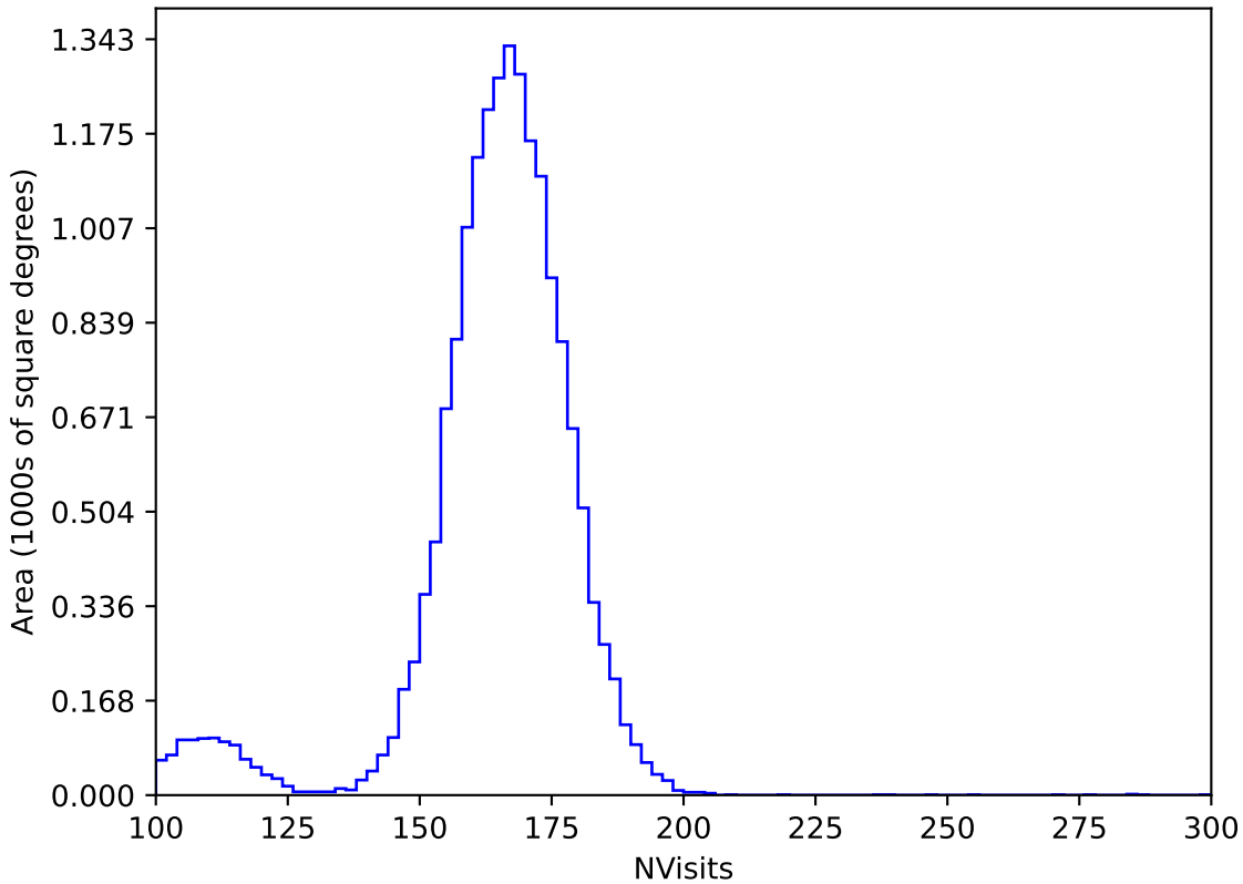
baseline_v3.0_10yrs WFD y band: NVisits
