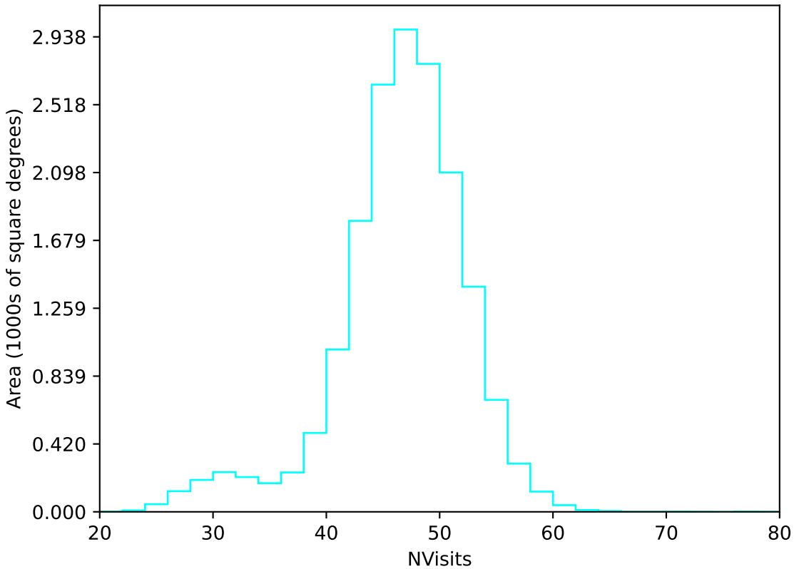
baseline_v3.0_10yrs WFD u band: NVisits
