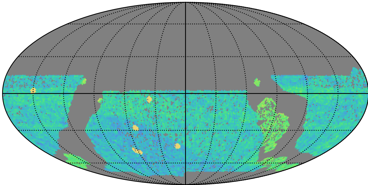
baseline_v3.0_10yrs WFD r band: NVisits
