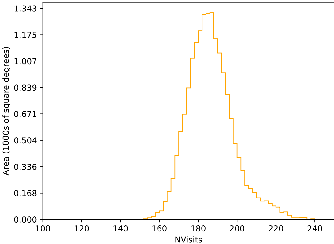
baseline_v3.0_10yrs WFD r band: NVisits
