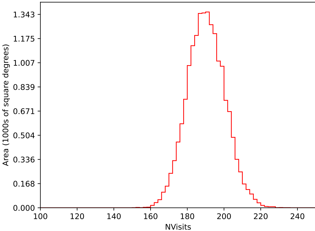
baseline_v3.0_10yrs WFD i band: NVisits
