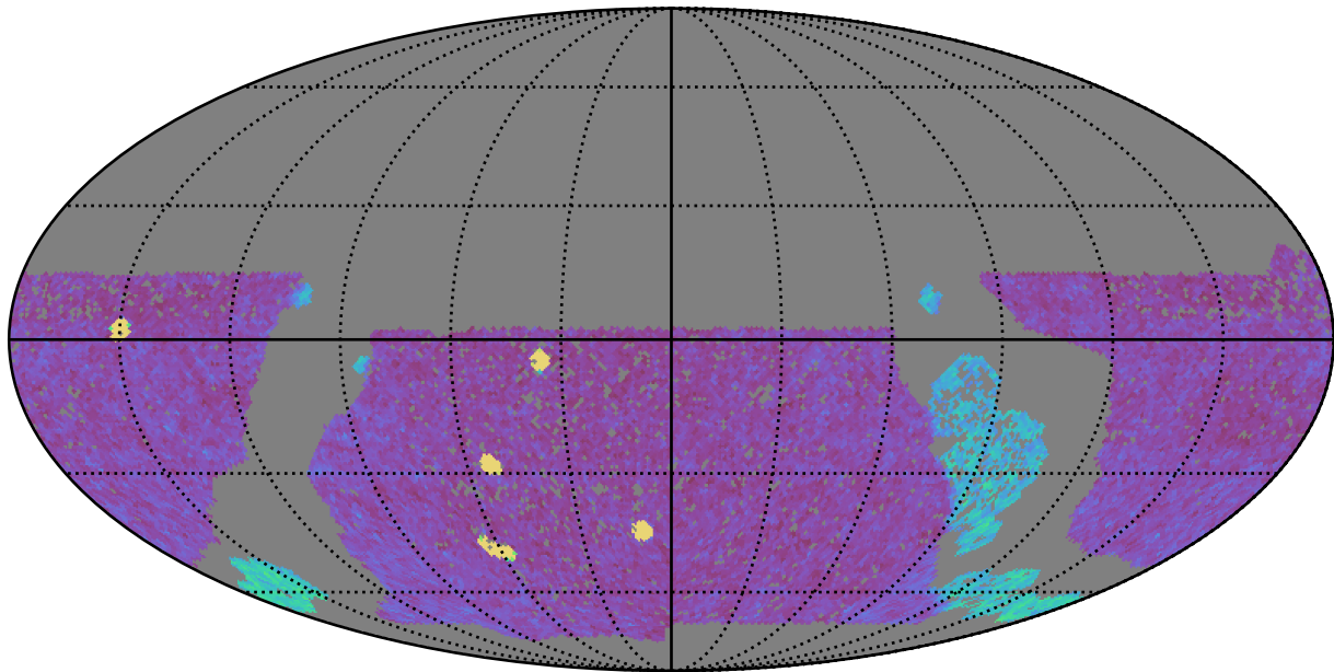
baseline_v3.0_10yrs WFD g band: NVisits
