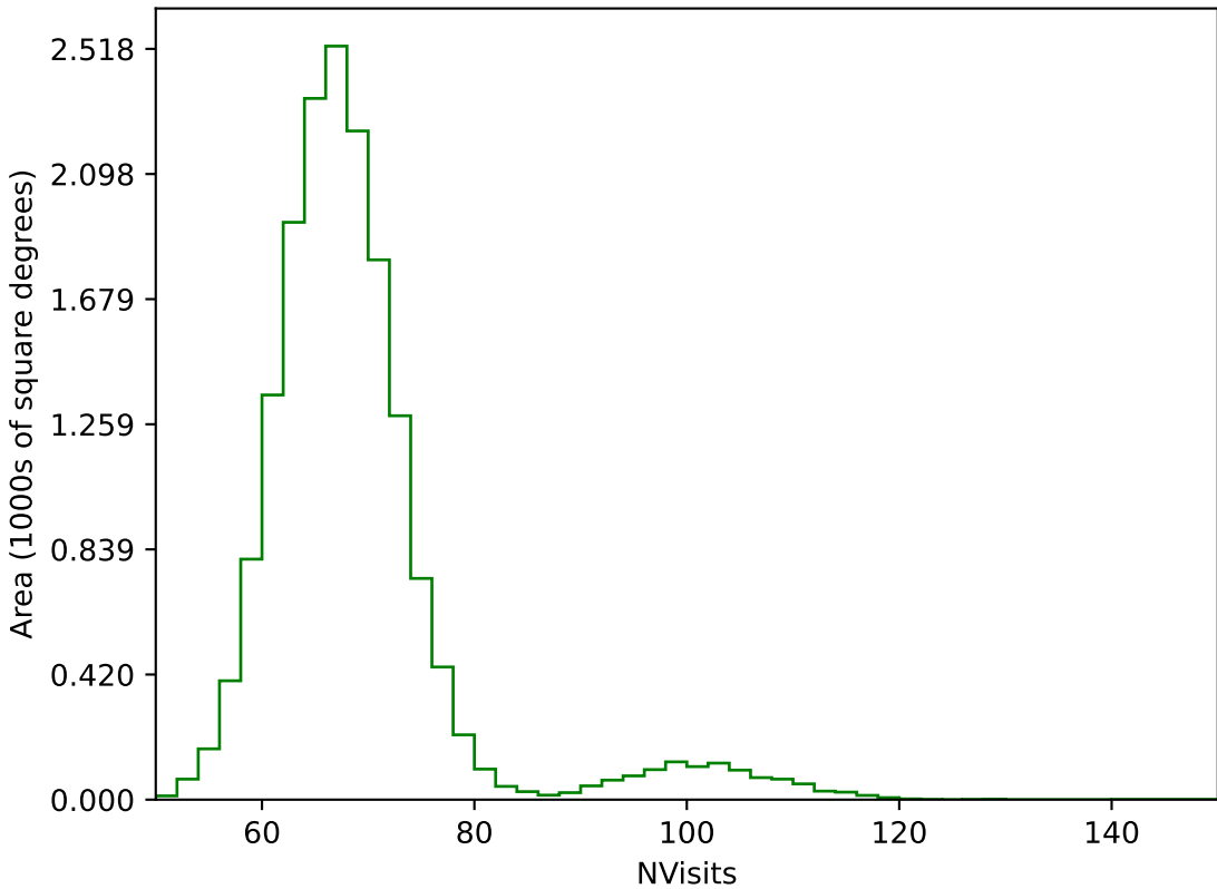
baseline_v3.0_10yrs WFD g band: NVisits
