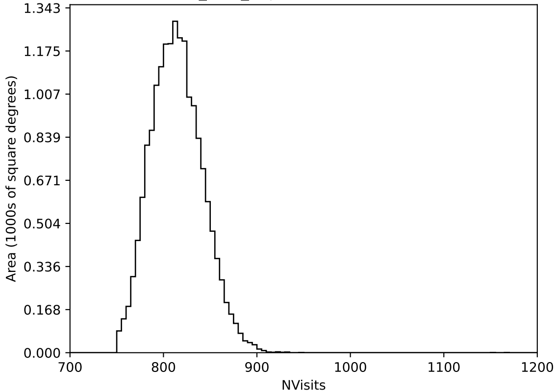
baseline_v3.0_10yrs WFD all bands: NVisits
