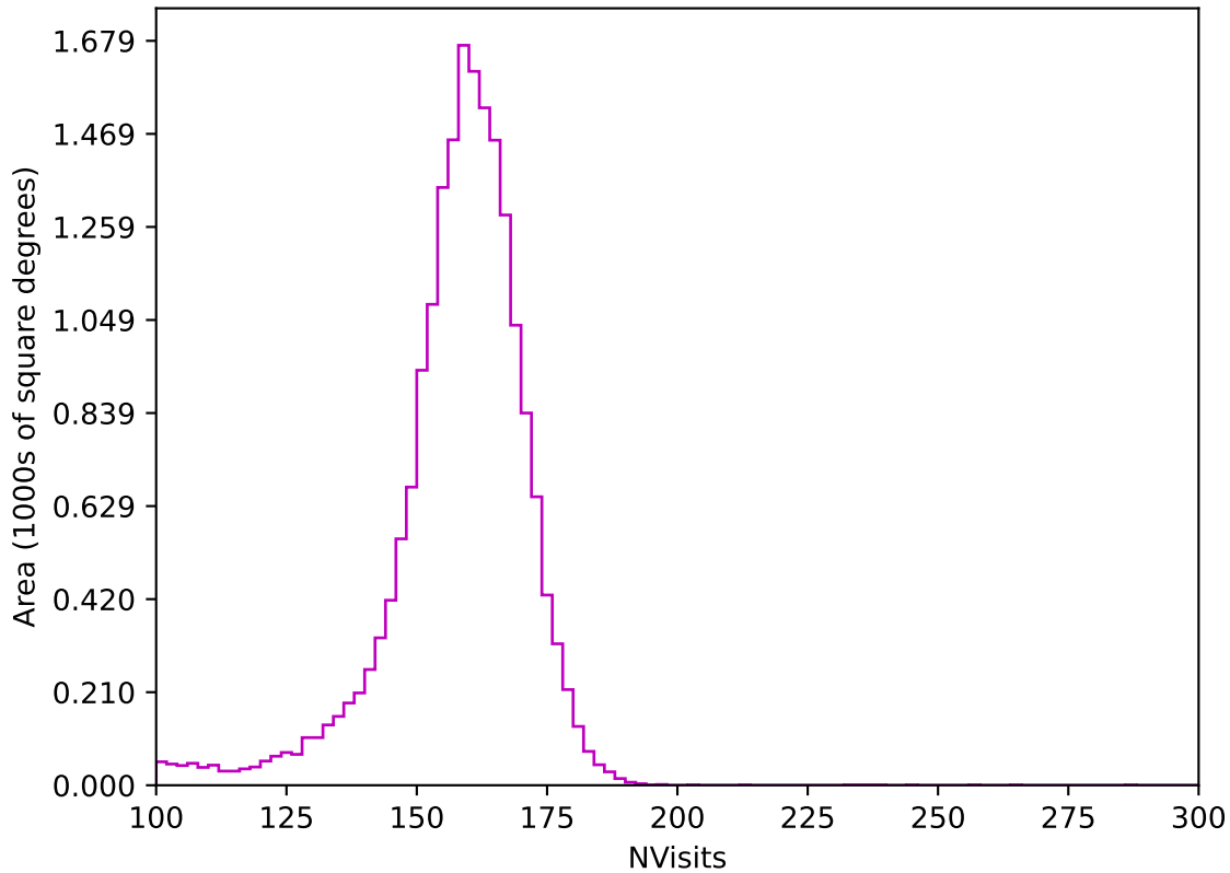
baseline_v3.0_10yrs All sky z band: NVisits
